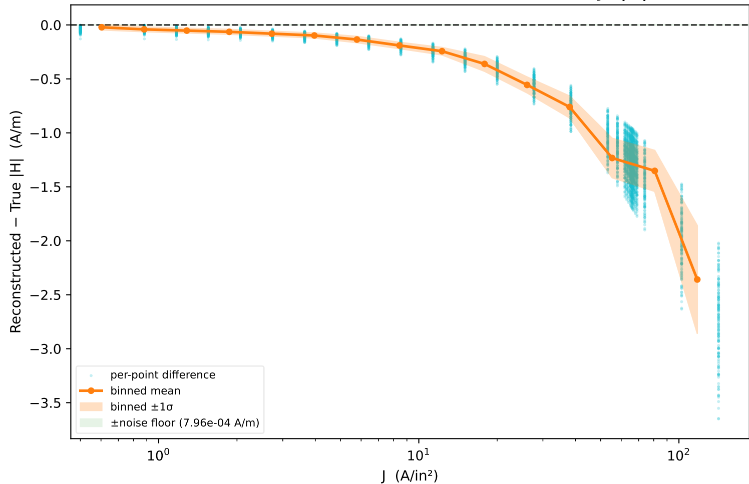
Reconstruction Error vs. Coil Current Density ( |H| )
